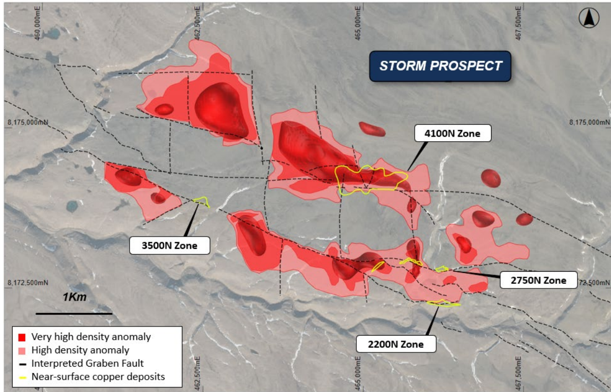
Figure 5: Gravity data interpretation map showing the 3D gravity targets, known copper sulphide deposits and major faults (overlying topography).
