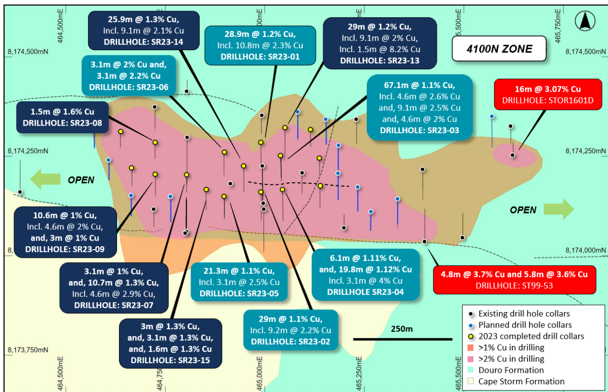
Figure 1: Plan view of the 4100N Zone showing interpreted copper mineralisation footprint (defined by historical drilling and EM), historical and recent drilling details, overlaying regional geology.
