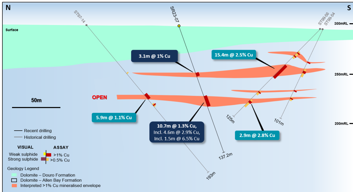
Figure 2: Geological section view at 464,800E showing the interpreted mineralisation envelopes (>0.5% & >1% Cu) and recent drill hole assays and visual observations.
