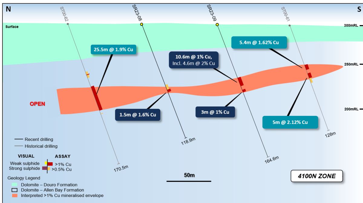
Figure 3: Geological section view at 464,725E showing the interpreted mineralisation envelope (>0.5 & >1% Cu) and recent drill hole assays and visual observations.
