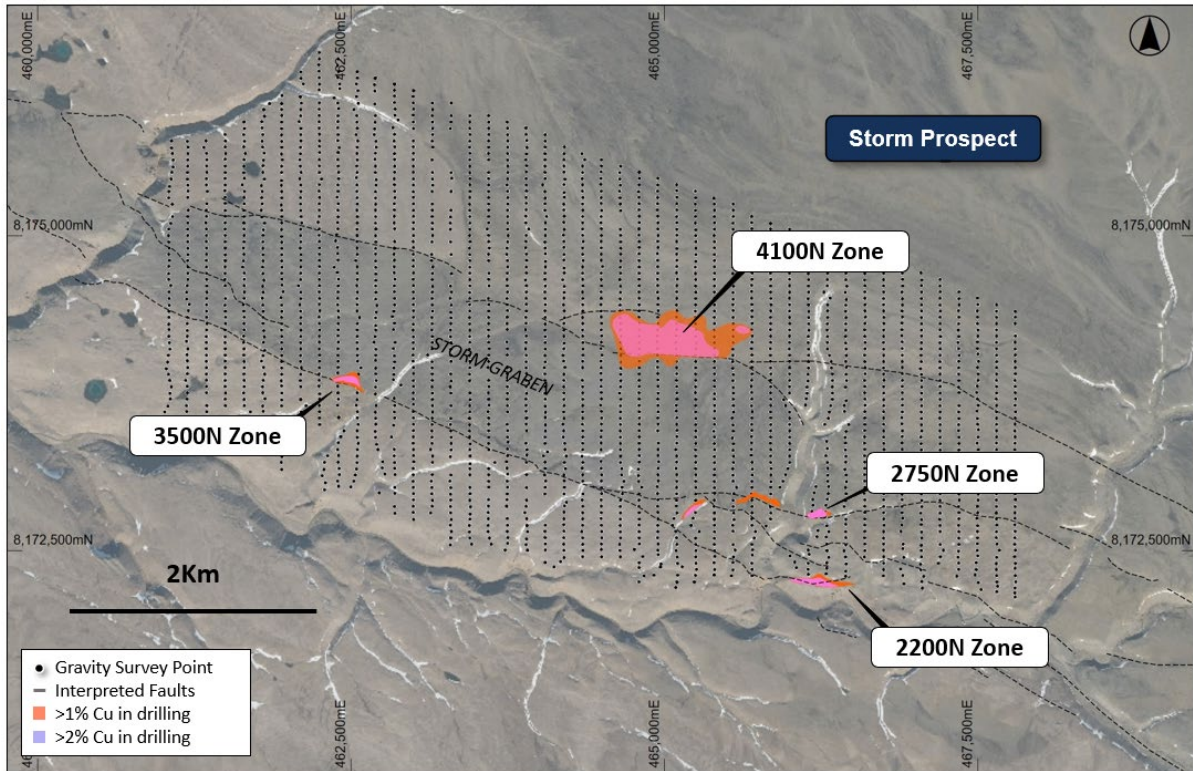
Figure 10: Plan view of the Storm Project area showing the completed ground gravity survey stations.
